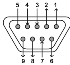
DB-9 Female
