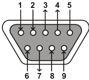
DB-9 Male
