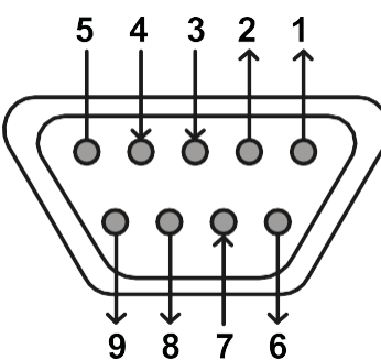
DB-9 Female
