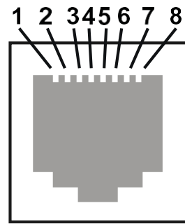
Rj-45 Jack (Female)
