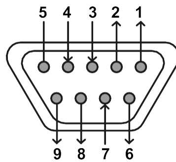
DB-9 Female
