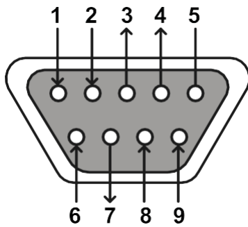
DB-9 Male
